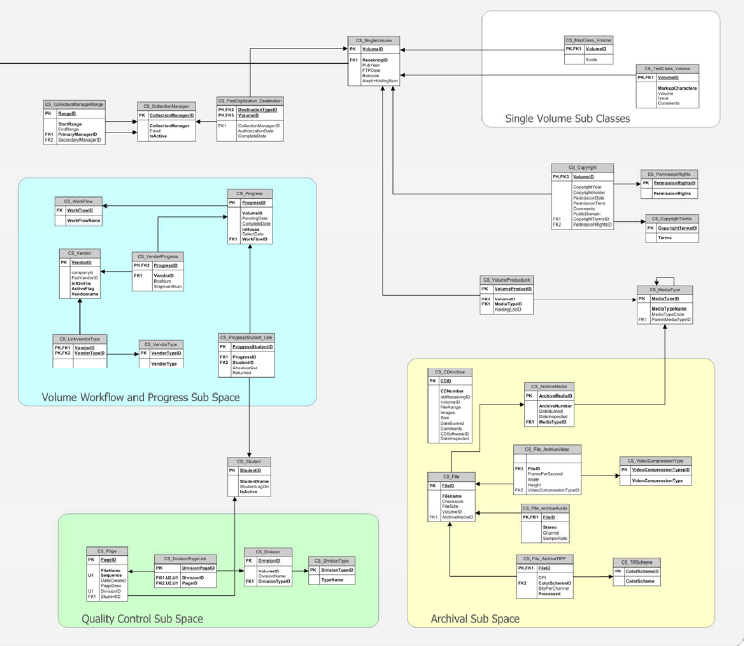
Tracking Database Rewrite SQL Database Diagram
